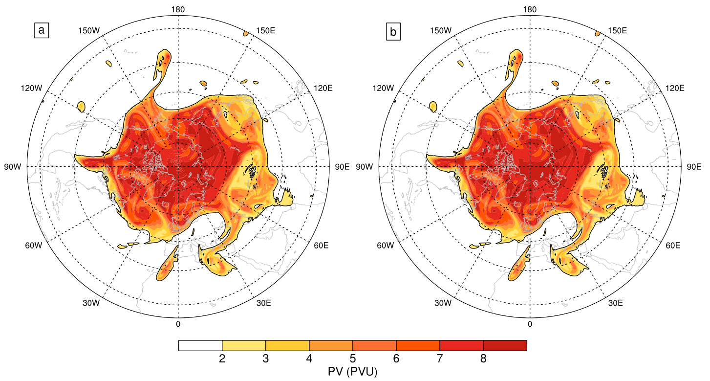
ERA5 reg05 Gibbs 1994-11-1, 0 UTC 330
