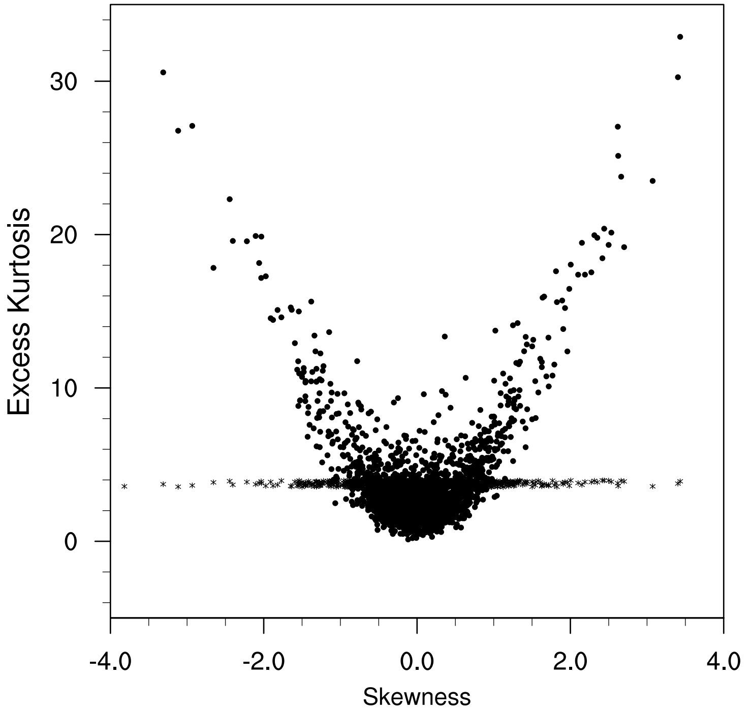
a) Hist Excess Kurtosis versus Skewness
