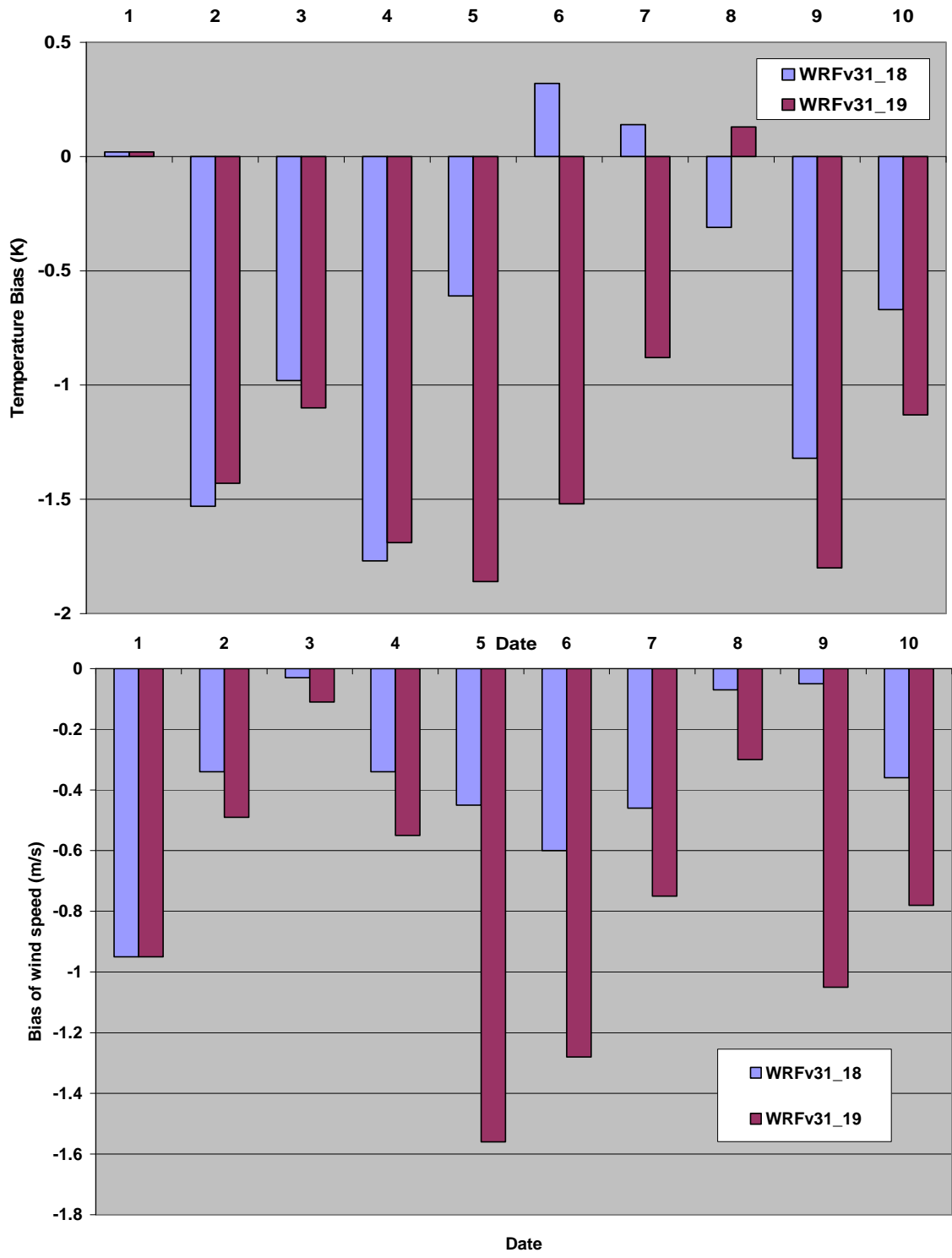
Upper panel: Temperature bias comparing against observations. Bottom panel: Wind speed bias comparing against observations
