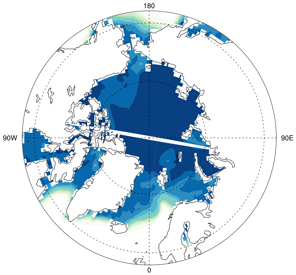
ice concentration (%)
