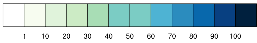
ice concentration (%)
