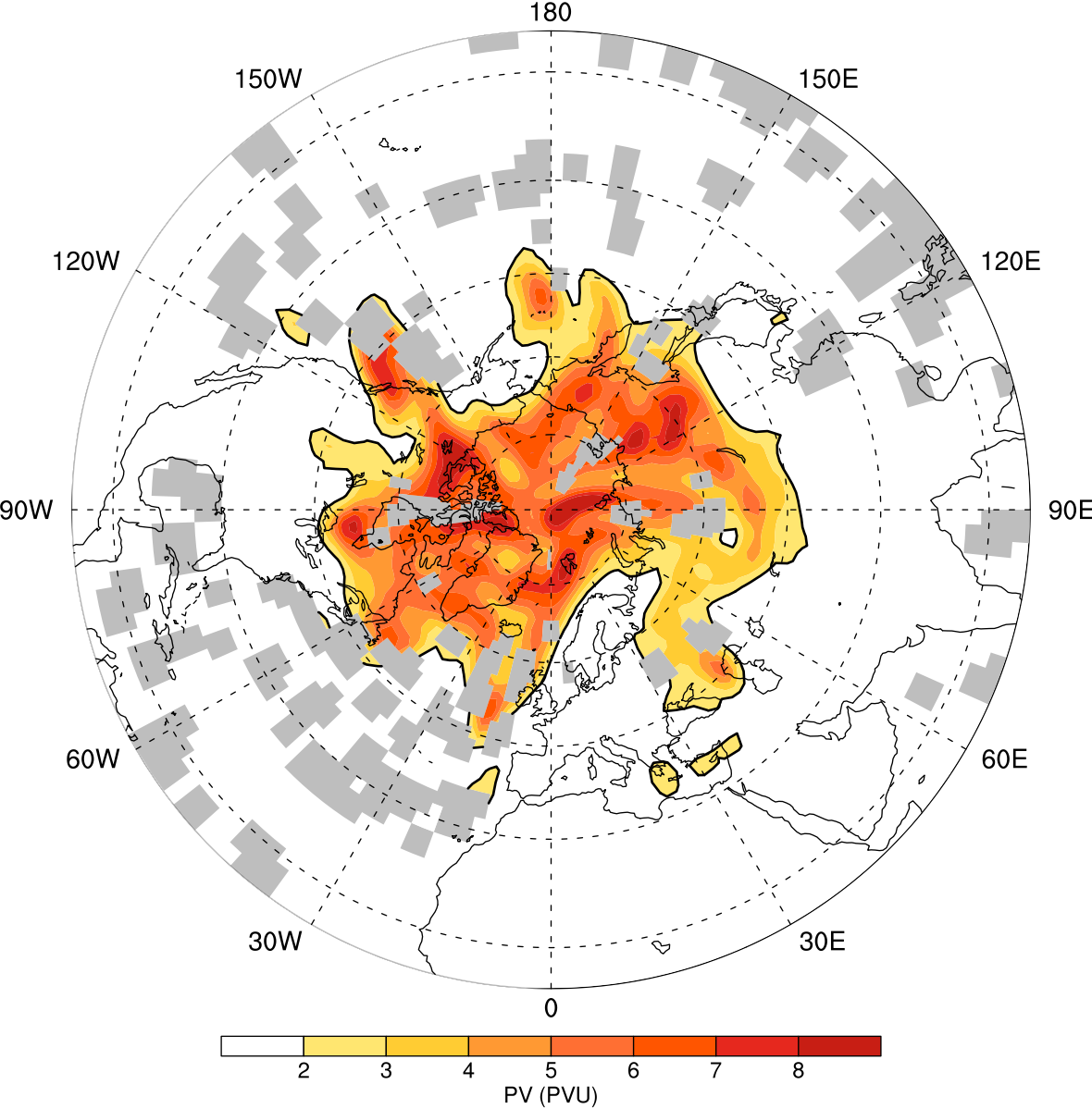
PV (330 K) 1 10 1937, 6 UTC (20CR ensemble mean, r2x2, computed)
