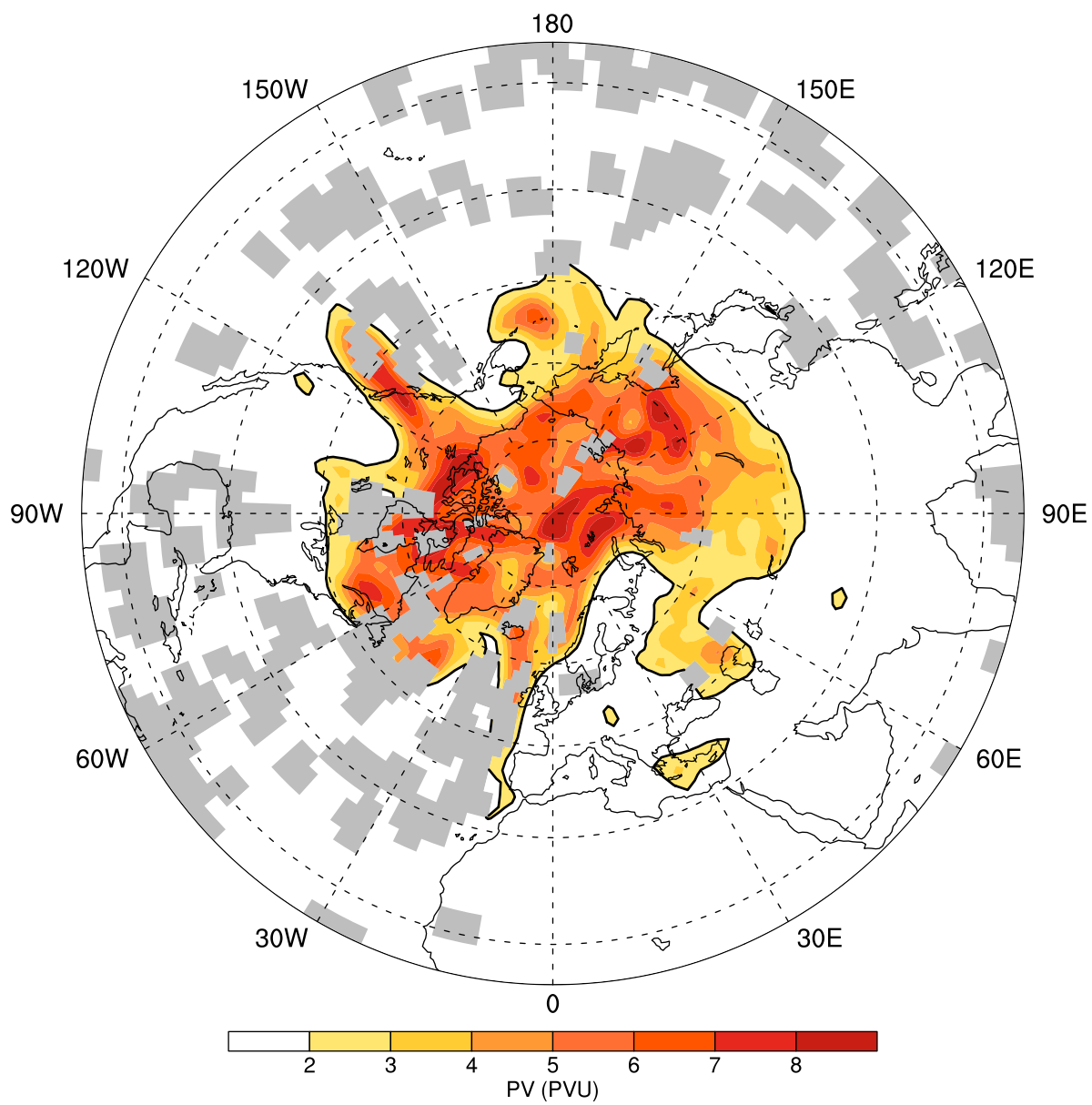
PV (330 K) 1 10 1937, 18 UTC (20CR ensemble mean, r2x2, computed)
