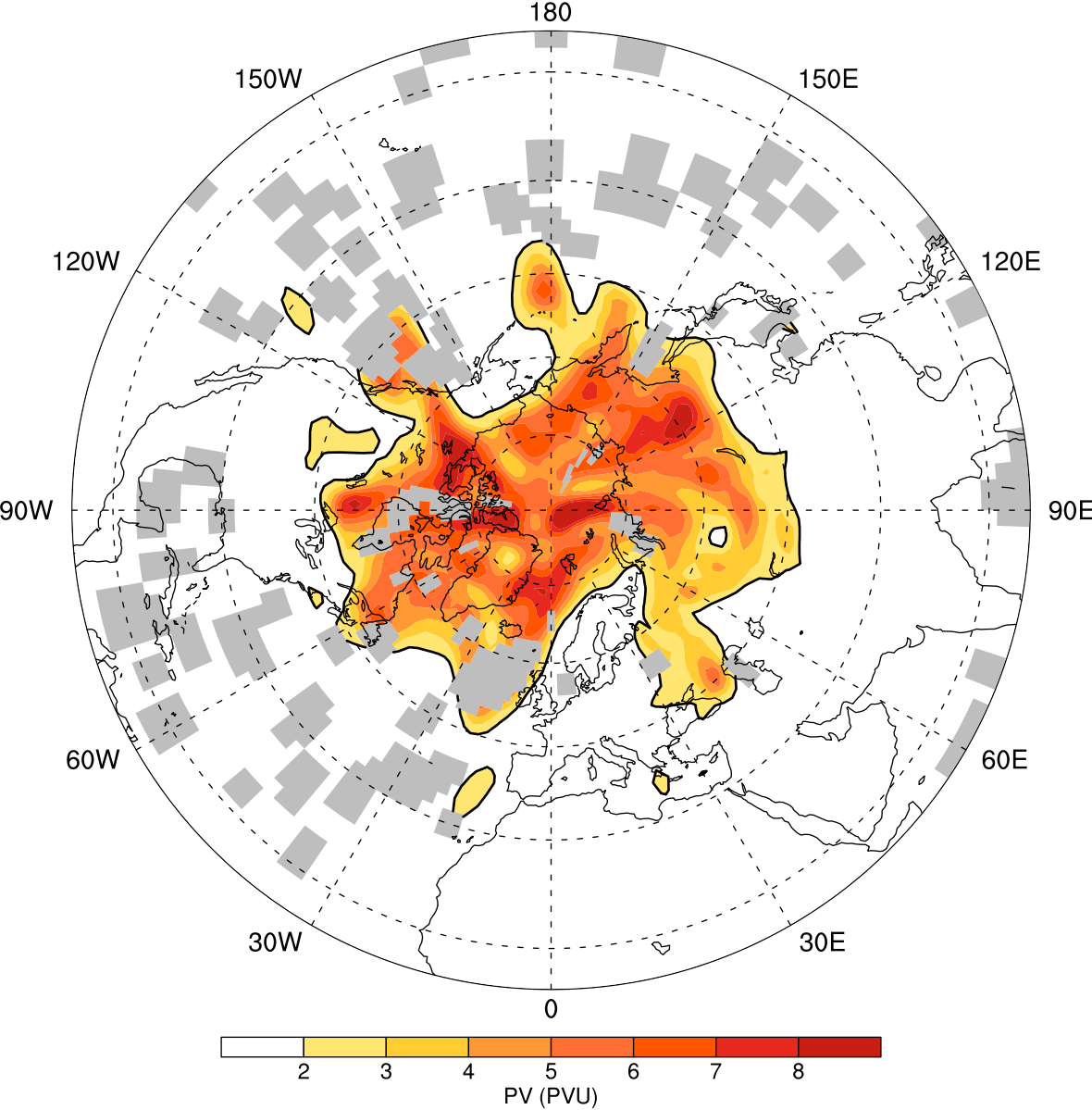
PV (330 K) 1 10 1937, 0 UTC (20CR ensemble mean, r2x2, computed)
