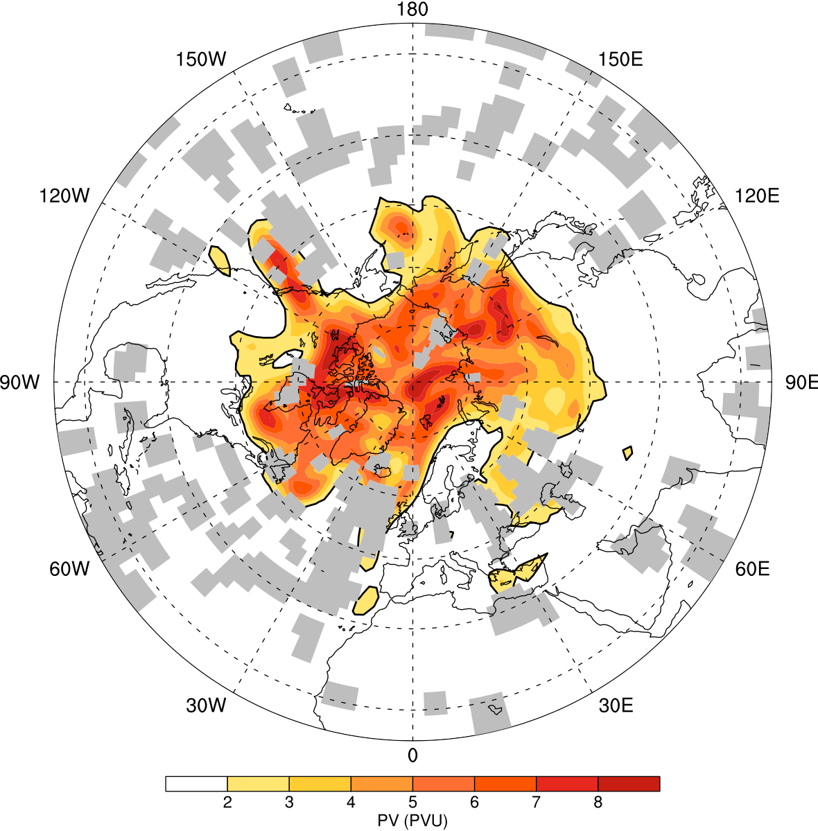
PV (330 K) 1 10 1937, 12 UTC (20CR ensemble mean, r2x2, computed)
