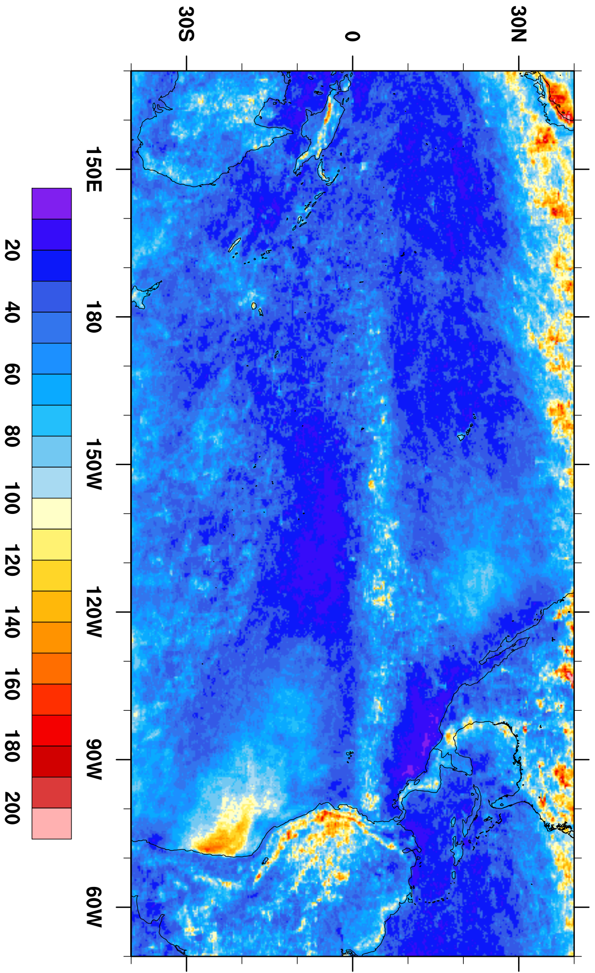
DECEMBER 2015: CLOUD LIQUID WATER PATH - LAYER 3 ( \text{g m}^{-2} ) CERES_SSF_Aqua-XTRK_Edition4A
