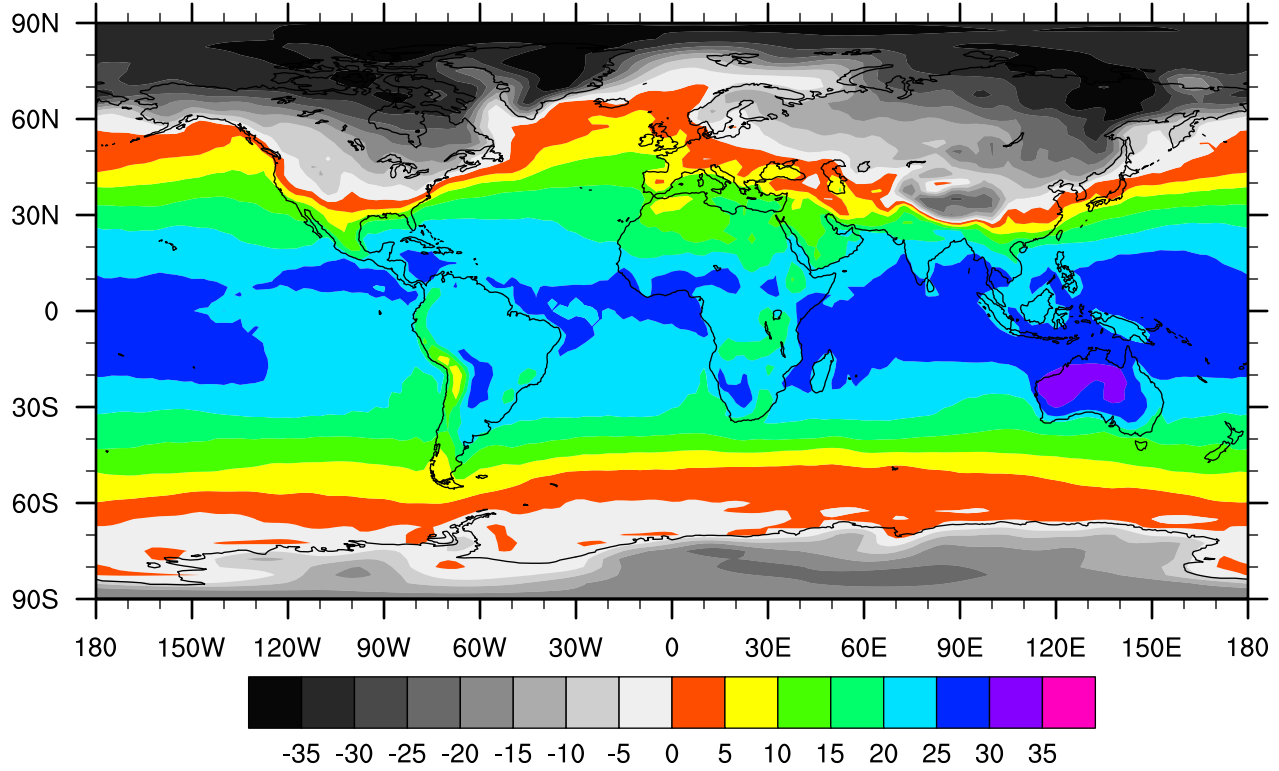
Monthly Mean Air Temperature at sigma level 0.995
