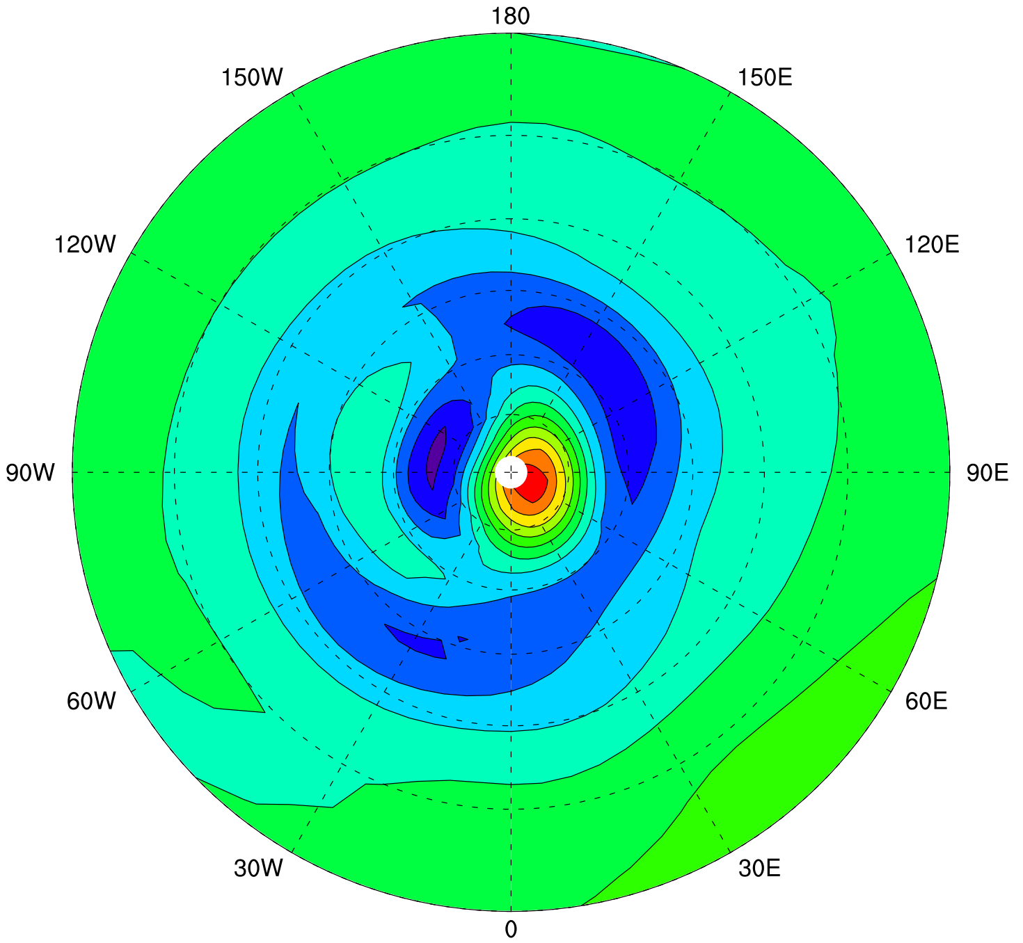
Temperature, with Kelvin Wave, 65 km altitude
