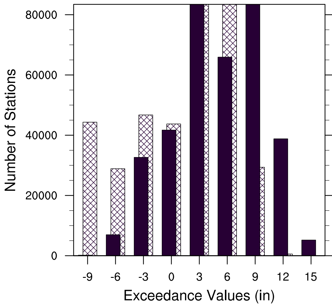
Obs vs WRF 4 km Ens.
