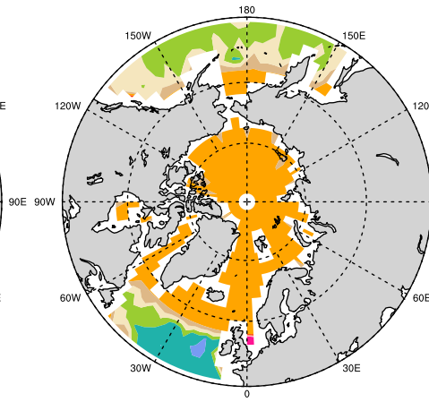
Bilinear
