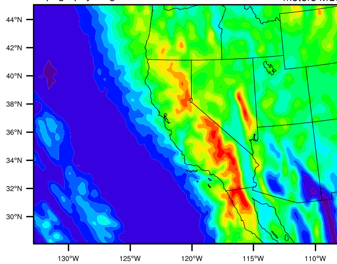
Topography height meters MSL
