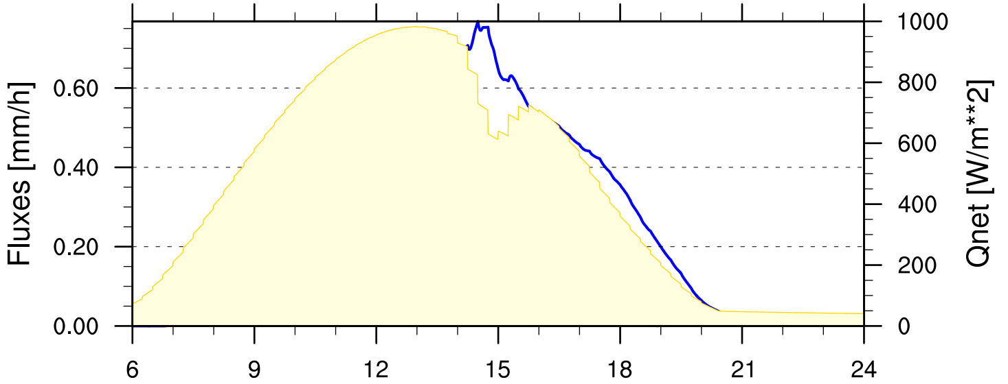
70% saturated soil | mean Bowen ratio=0.63
