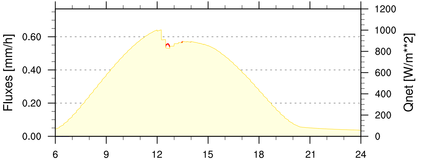
40% saturated soil | mean Bowen ratio=118.36
