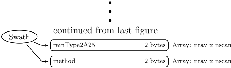
Figure 84: Data Format Structure for 2H25, Spectral Latent Heating
