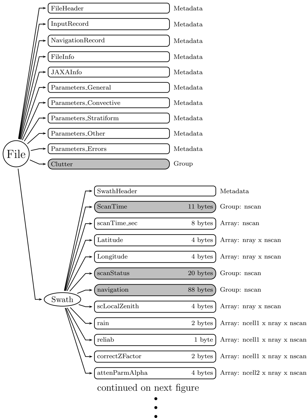
Figure 45: Data Format Structure for 2A25, PR Profile
