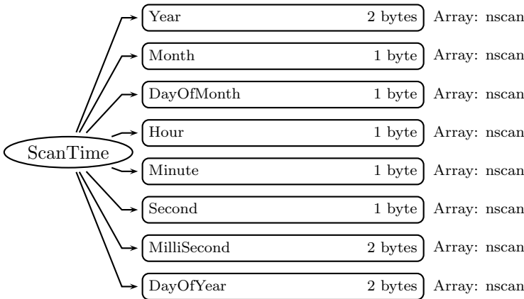
Figure 85: Data Format Structure for 2H25, ScanTime
