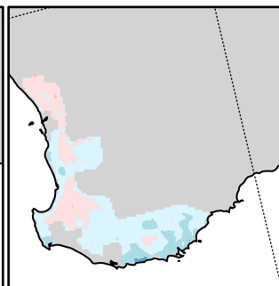
(f) ERA-Interim bias
