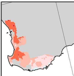
(g) CCSM bias
