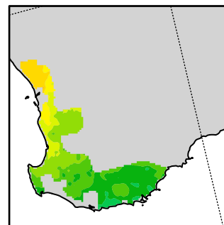
(e) ECHAM
