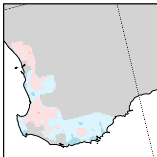
(e) ECHAM
