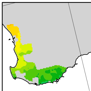
(c) CCSM
